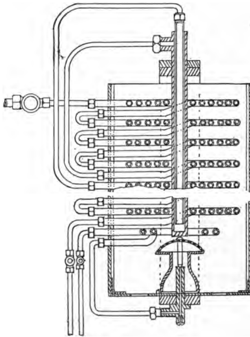
FIG. 349.—Sectional Elevation of the Blaxton Flash Generator.
